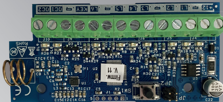
webeyeFOG Transmitter
